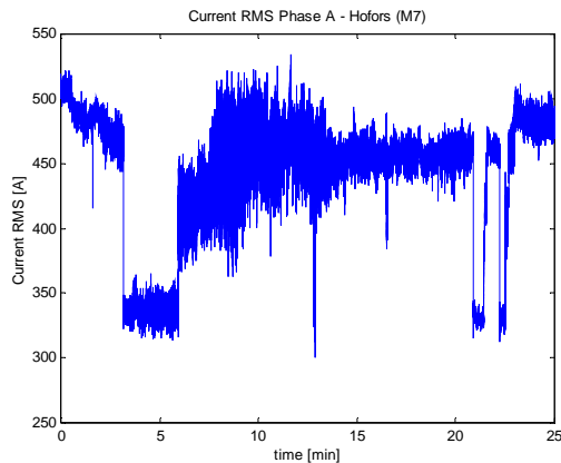
Fig. 6. Diagram of the RMS current of the outgoing line to Hofors (M7). The heavy fluctuation that starts after 6 minutes is certainly due to the operation of the arc furnace located in Hofors. The fluctuations in current will result in flicker power fluctuations shown in Fig. 5 c.
