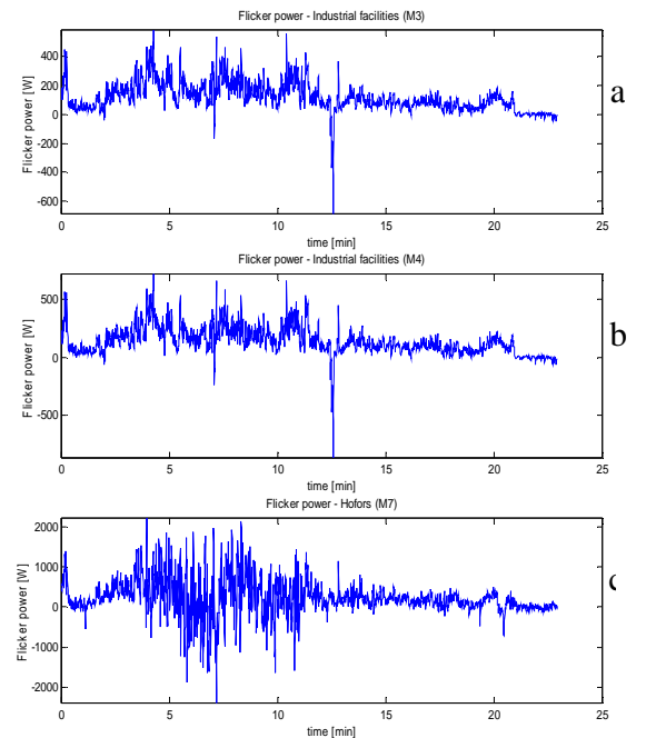
Fig. 5. Measurement results from monitoring points producing mainly positive flicker power.
