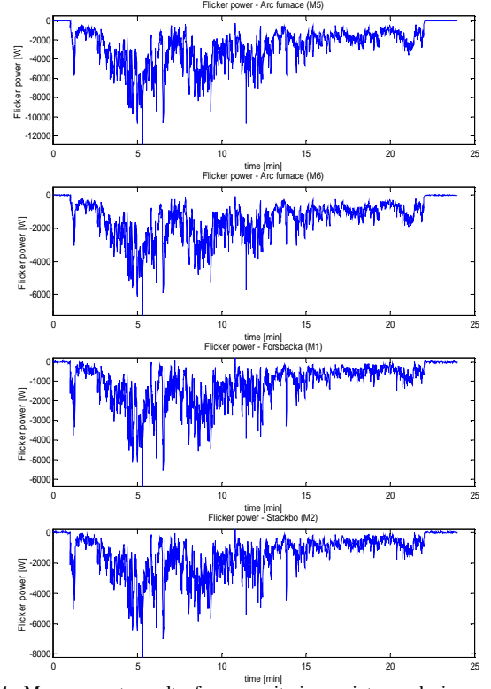
Fig. 4. Measurement results from monitoring points producing negative flicker power. Diagram a) and b) show the flicker power measured at the lines feeding the arc furnace and diagram c) and d) show the flicker power flowing in the incoming lines.
