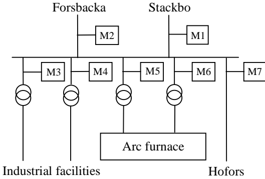
Fig. 3. One-line diagram of the 130 kV substation in Sandviken, Sweden.
