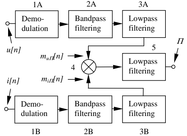
Fig. 2. Signal flow diagram of the proposed method.
