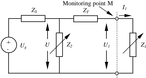
Fig. 1. Circuit model used to derive the proposed method.
